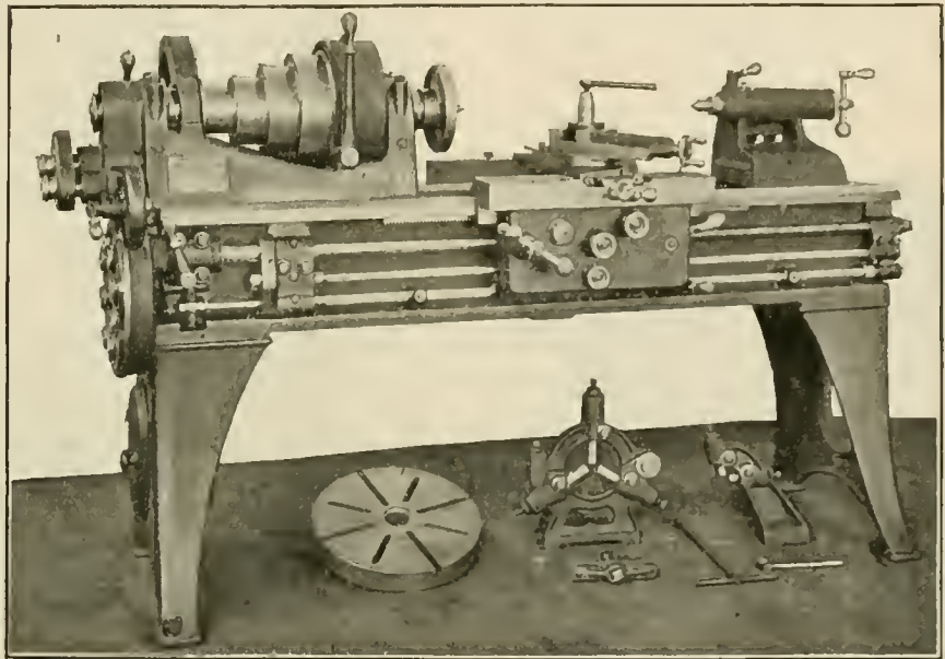
16-INCH IDEAL ENGINE LATHE.
